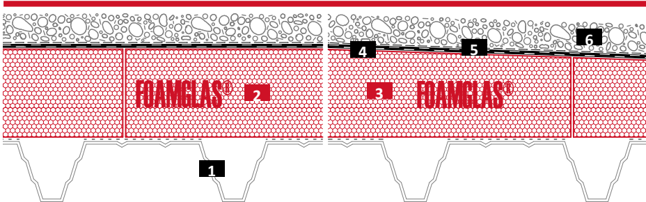
Schematic drawing
