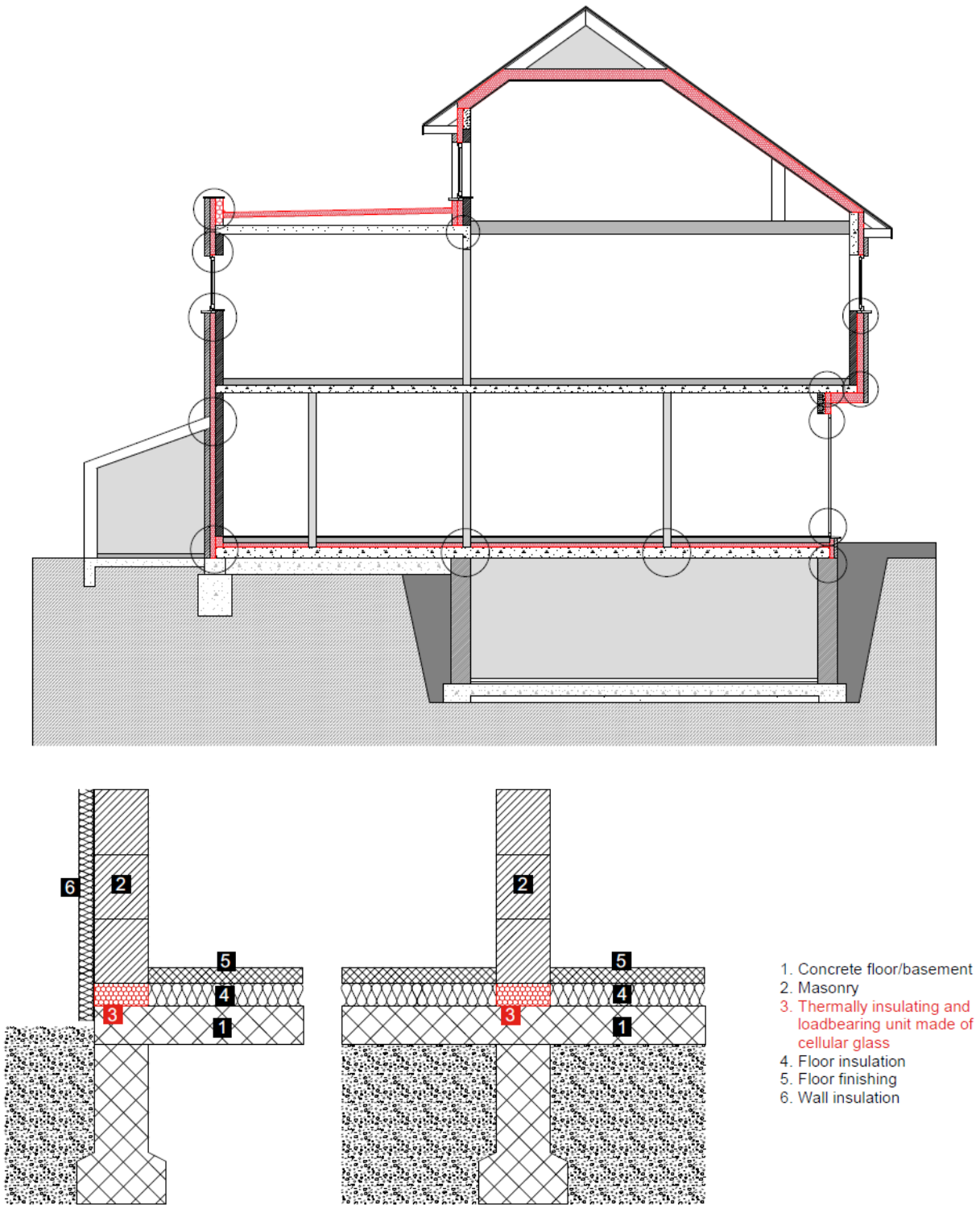
Figure 1: Example of the application of the thermally-insulating and loadbearing units of cellular glass
