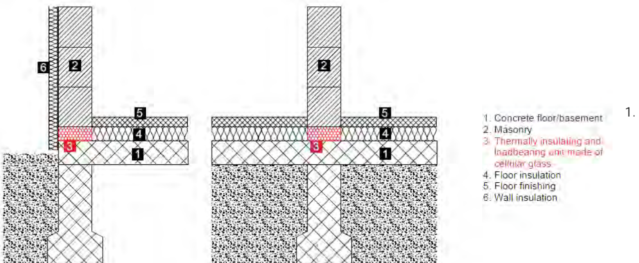
Figure 1: Example of the application of the thermally-insulating and loadbearing units of cellular glass
