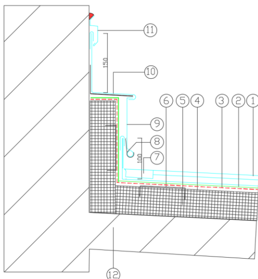
Figure 24 – Faîtage adossé
