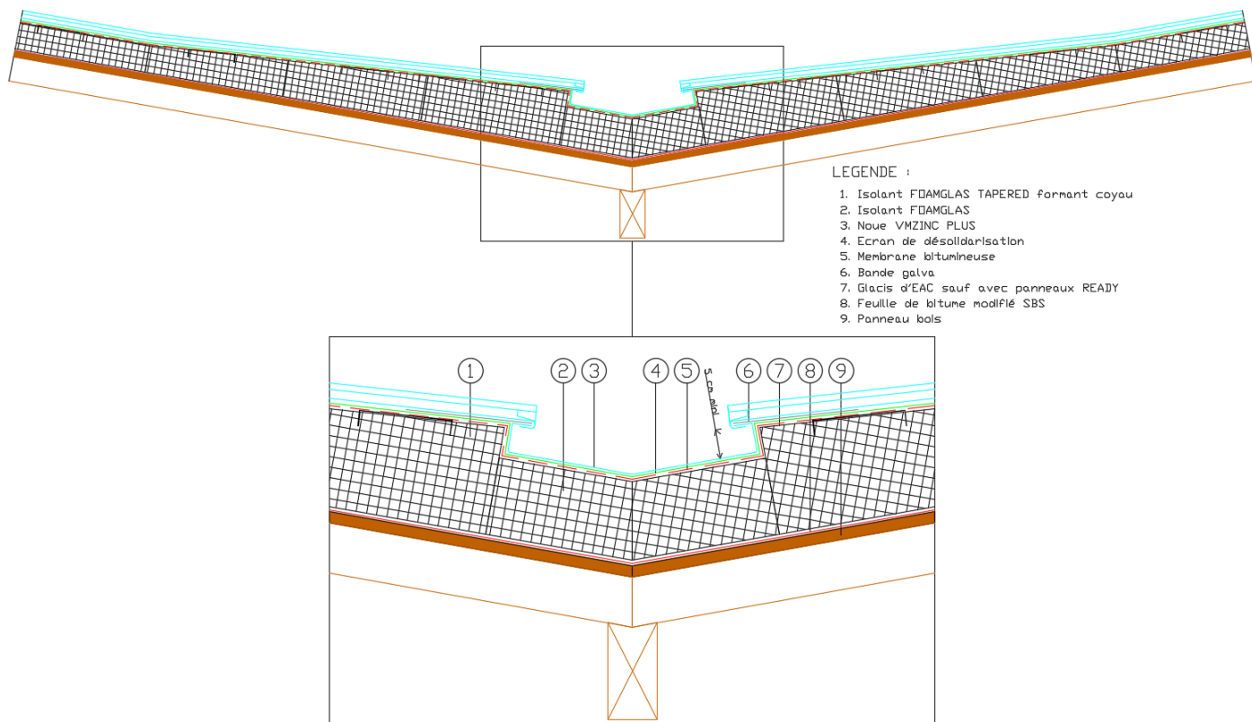
Figure 28 – Noue encaissée
